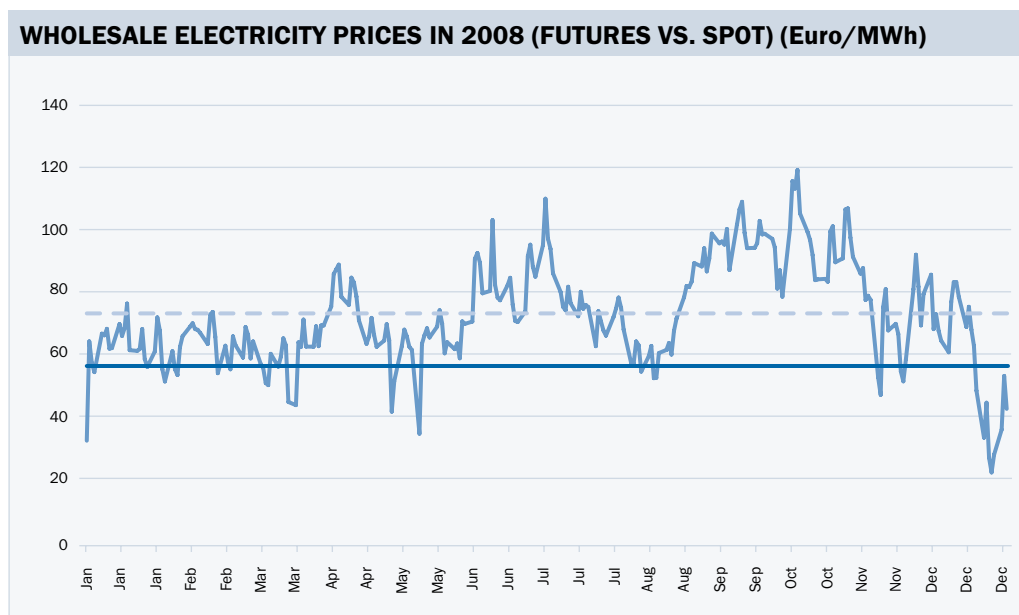
Figure 10 Wholesale electricity prices in 2008
